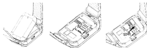
Open the battery cover T-flash card installation SIM card installation
